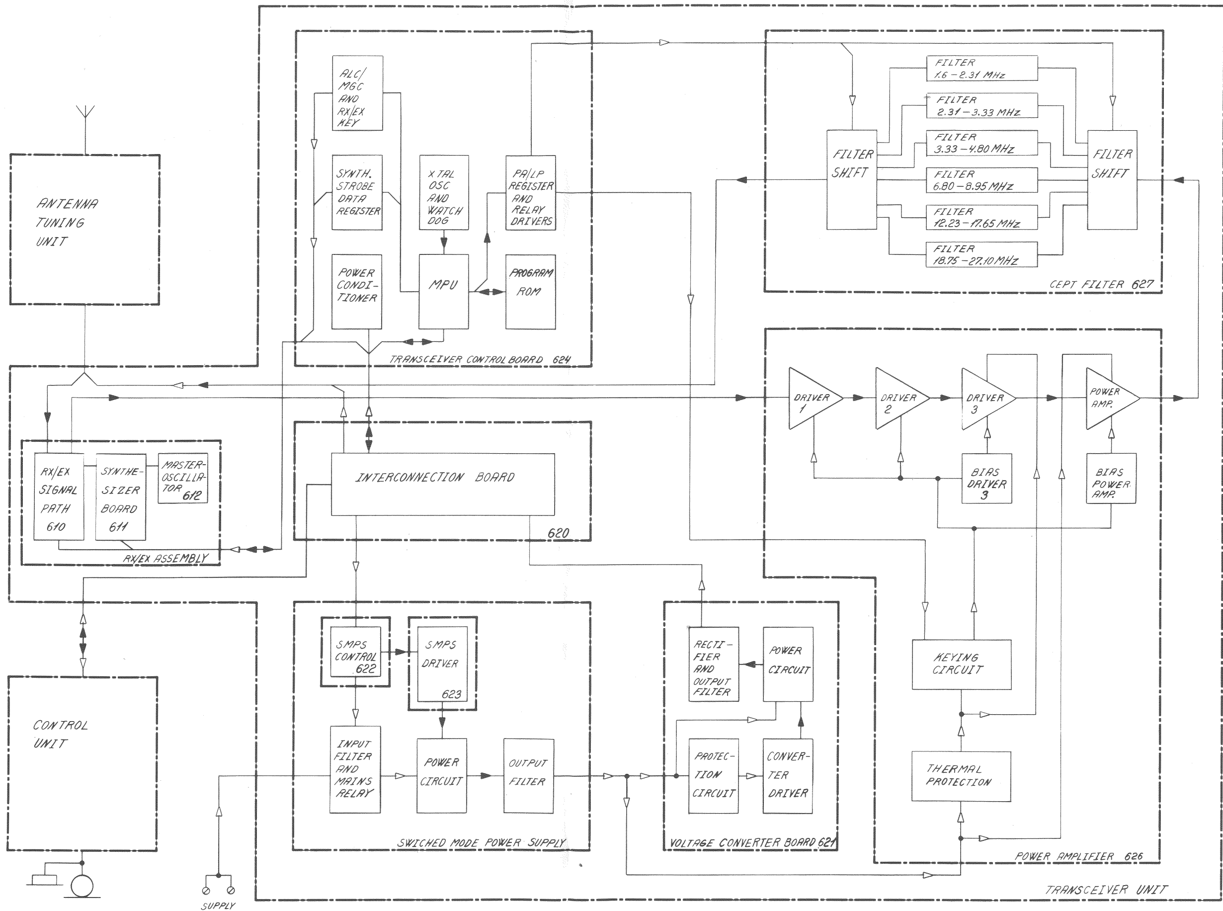
TRP8250S BLOCK DIAGRAM, TRANSCEIVER UNIT VERSION 1A
